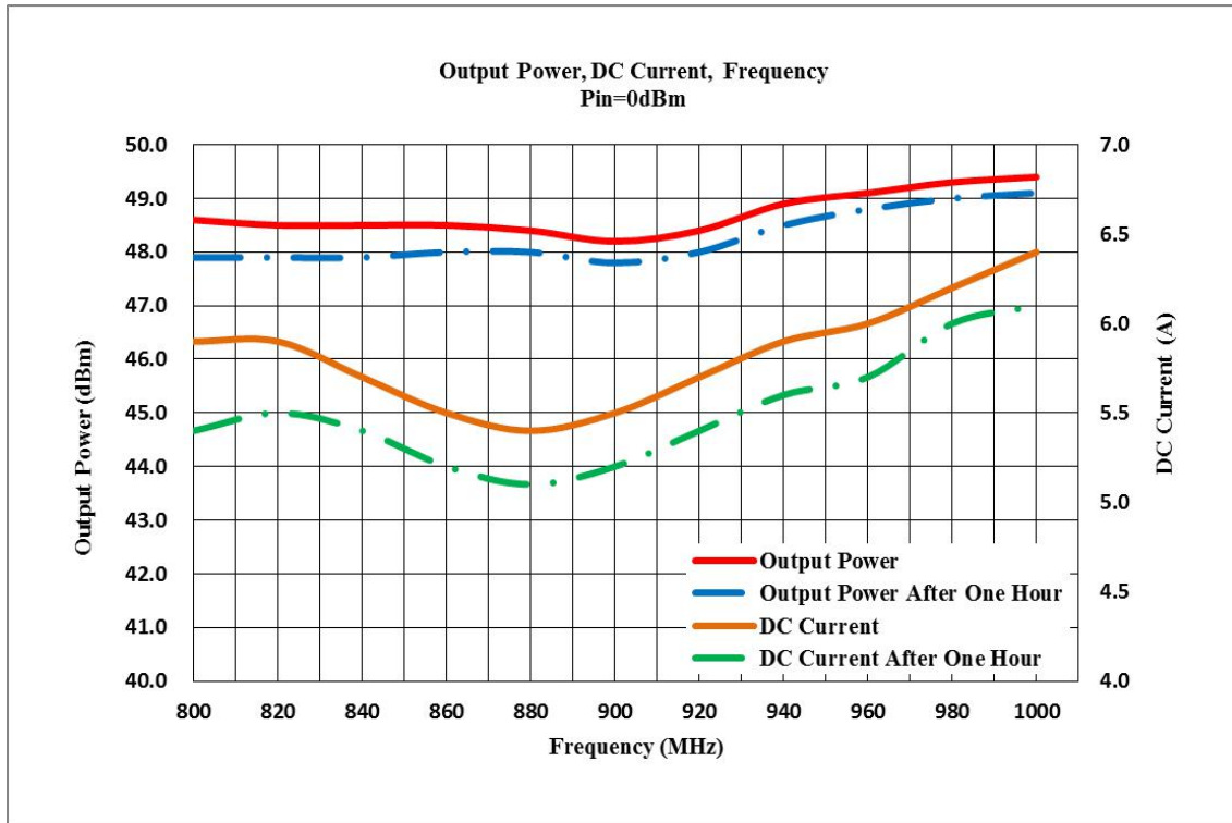
Graph2: Output Power(High temp.+60±3℃)
