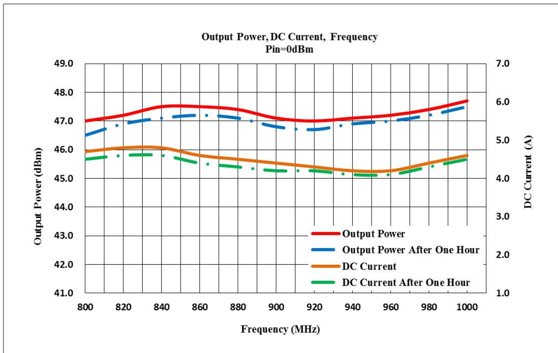
Graph2: Output Power(High temp.+60±3℃)
