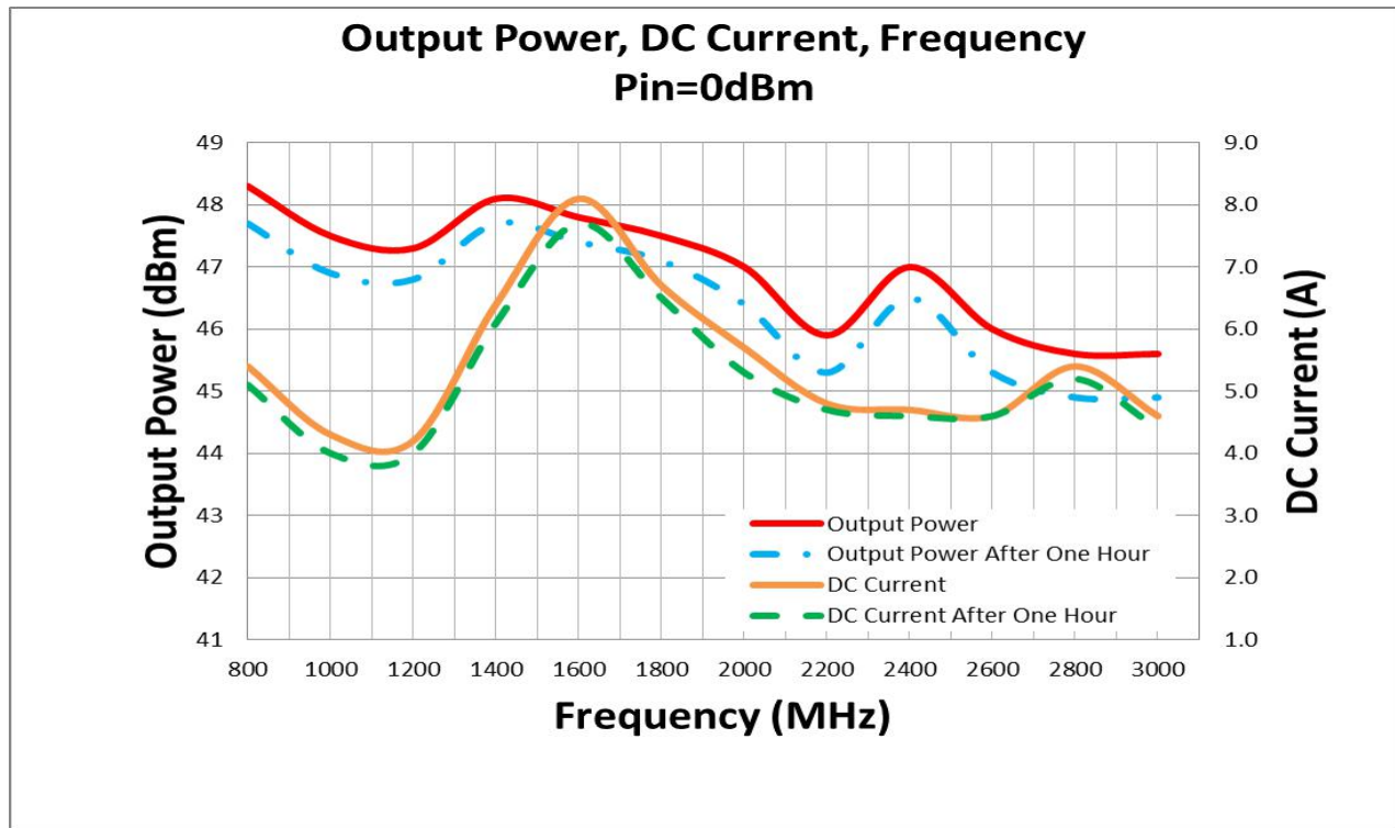
Graph2: Output Power (High temp. +65±3°C)
