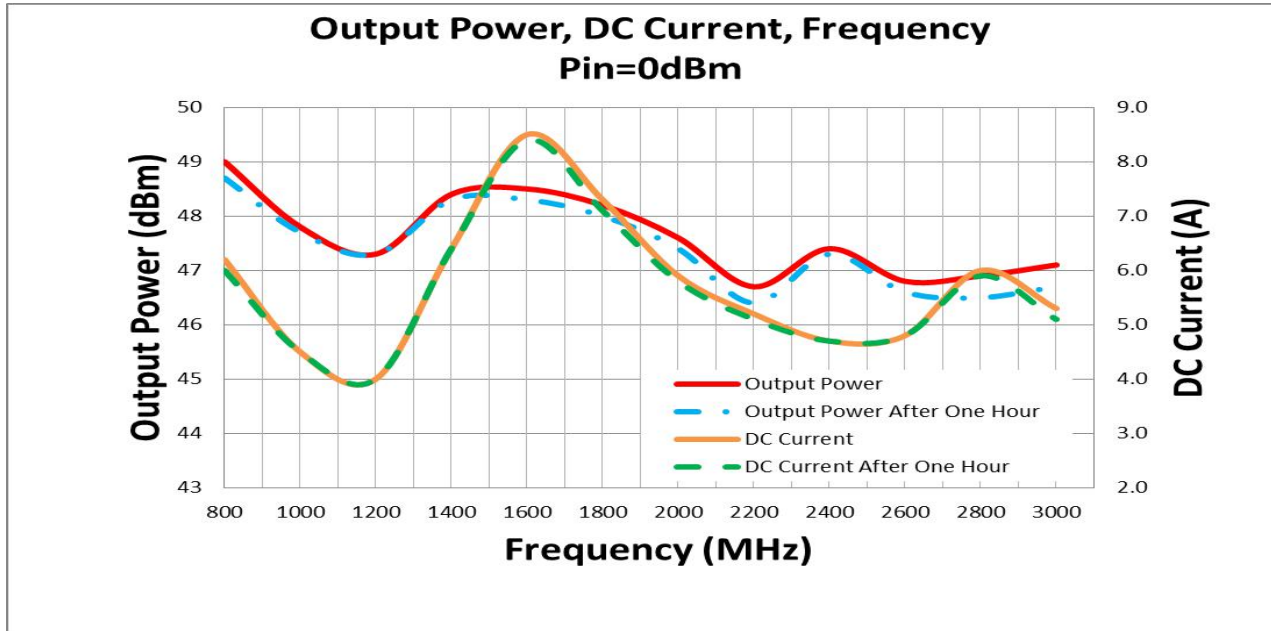
Graph2: Output Power (High temp. +65±3°C)
