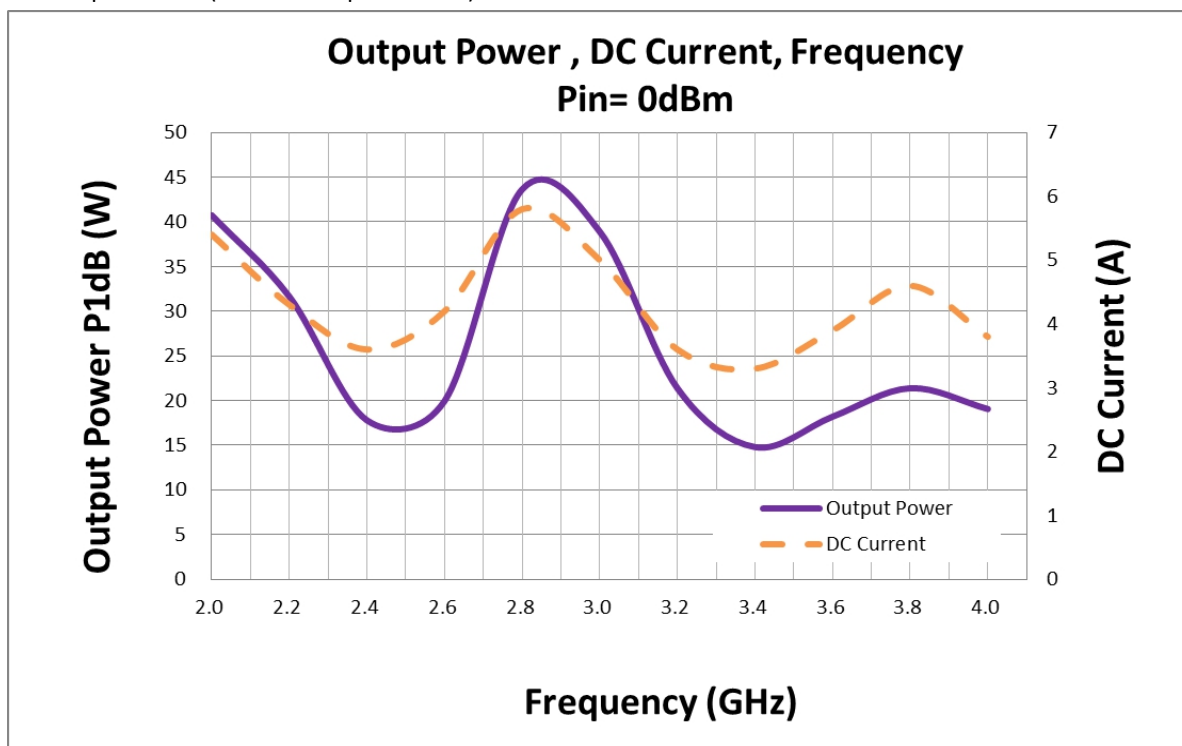
Graph 3: Output Power (Normal temp. +25\pm 3^{\circ}\text{C} )
